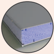
Panneau sandwich R = 0.28 m 2 .K/W
